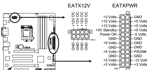
H87M-PLUS ATX power connectors
