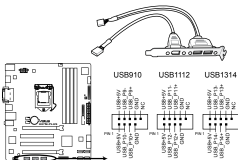
H87M-PLUS USB2.0 connectors
