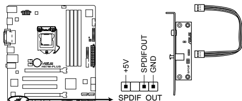
H87M-PLUS Digital audio connector
